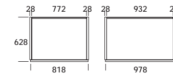
7- ANTA SCORREVOLE "MUST" - "REFLEX". "MUST" - "REFLEX" SLIDING DOOR. PUERTA CORREDERA "MUST" - "REFLEX".
