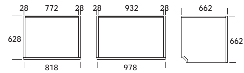
2- ANTA SCORREVOLE 2 SETTORI. SLIDING DOOR WITH 2 SECTIONS. PUERTA CORREDERA 2 SECTORES.
