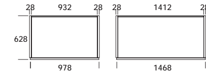
8- ANTA SCORREVOLE "MAGNUS". "MAGNUS" SLIDING DOOR. PUERTA CORREDERA "MAGNUS".
